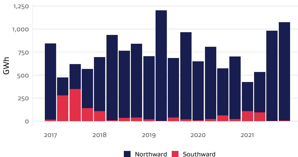
Figure C.3 Transfer of electricity by the High Voltage Direct Current (HVDC) inter-island link
