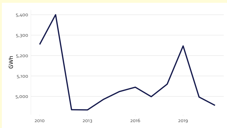
Figure C.5 Electricity use at Tiwai Point grid exit point
