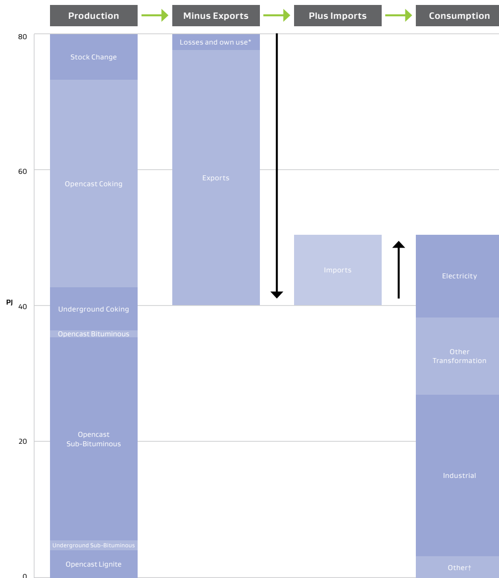
Figure C.2: Coal Energy Flow Diagram for 2016
