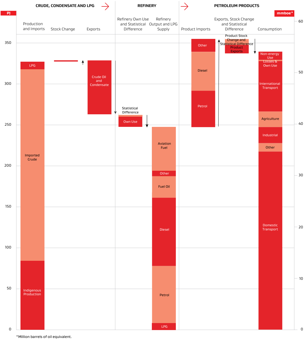
Figure D.2: Oil Energy Flow Summary for 2016
