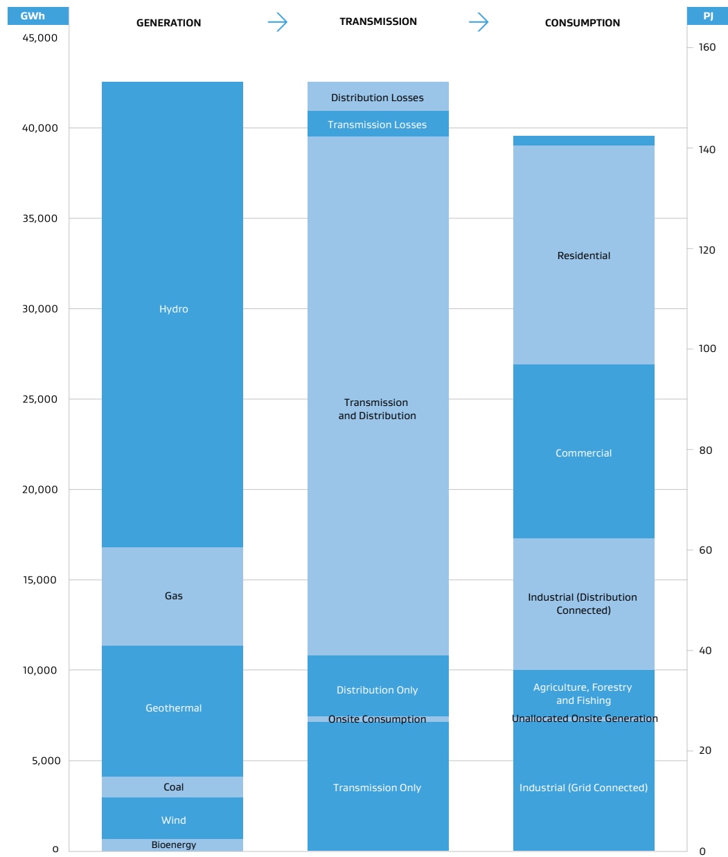
Figure F.2: Electricity Flow Diagram for the 2016 Year
