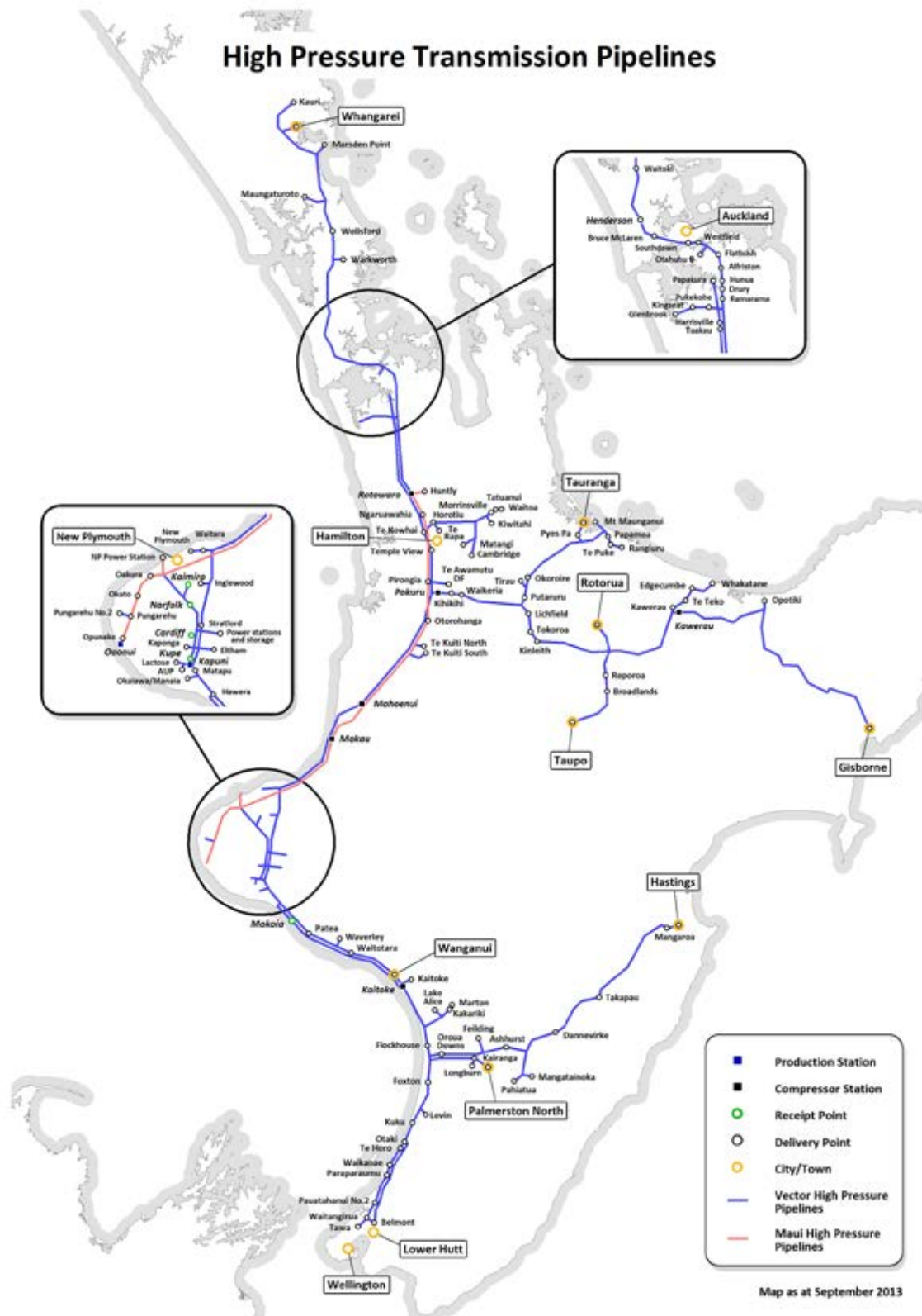
Figure D.10: New Zealand Natural Gas Transmission Pipeline
