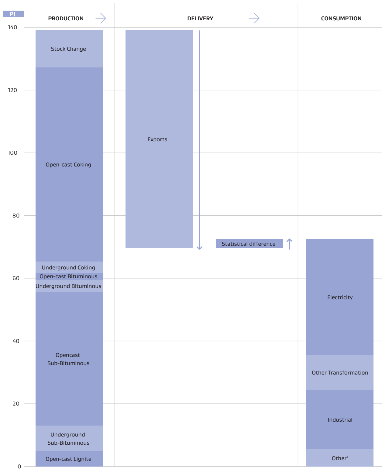
Figure C.6: Coal Energy Flow Diagram for 2012
