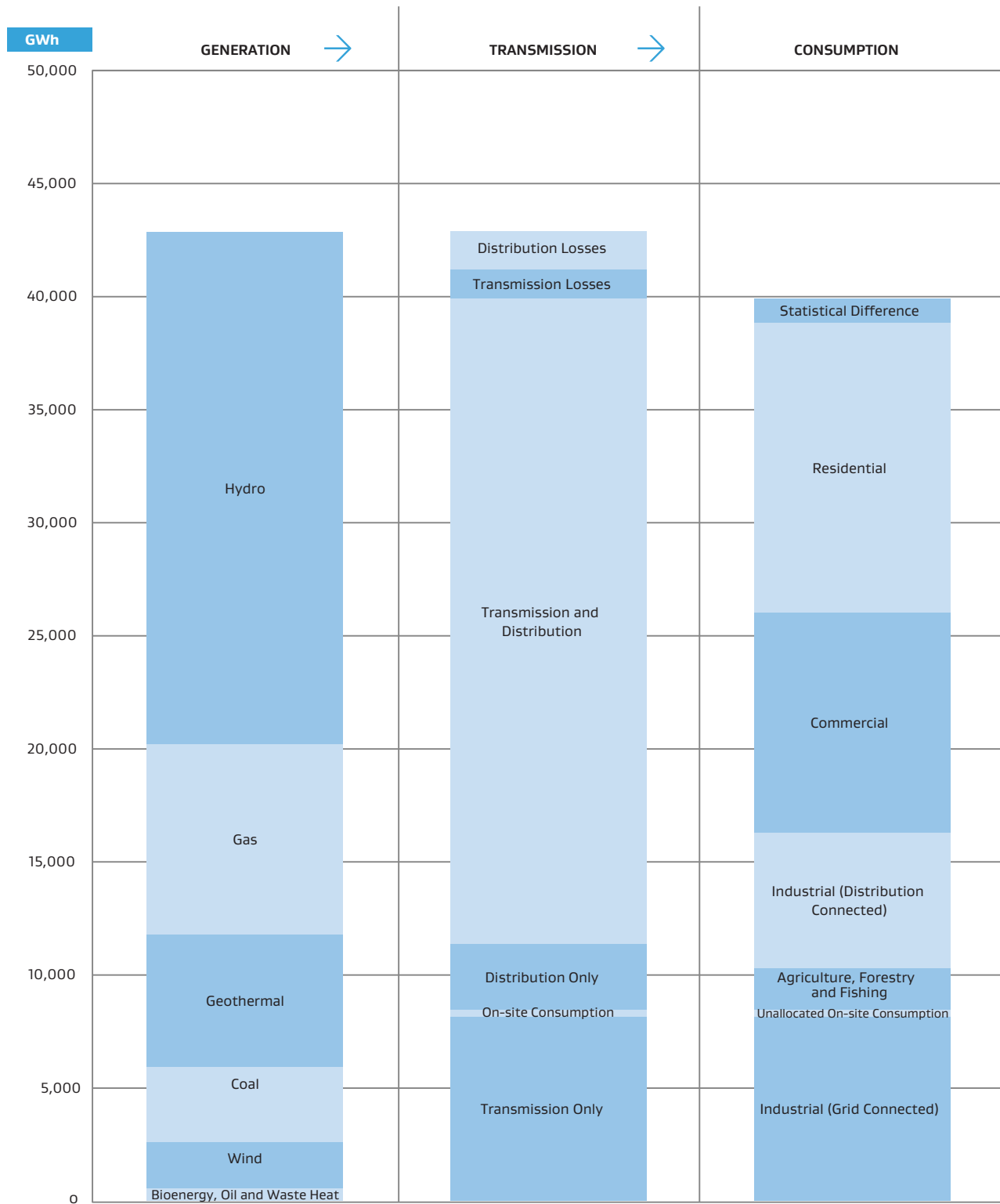
Figure F.1b: Electricity Flow Summary for 2012
