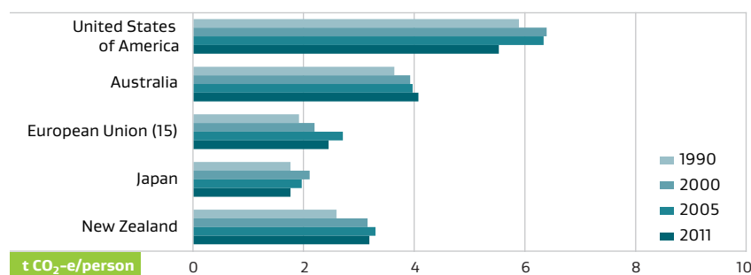
Figure A.5c: Transport Greenhouse Gas Emissions per Capita of Selected Annex 1 Countries
