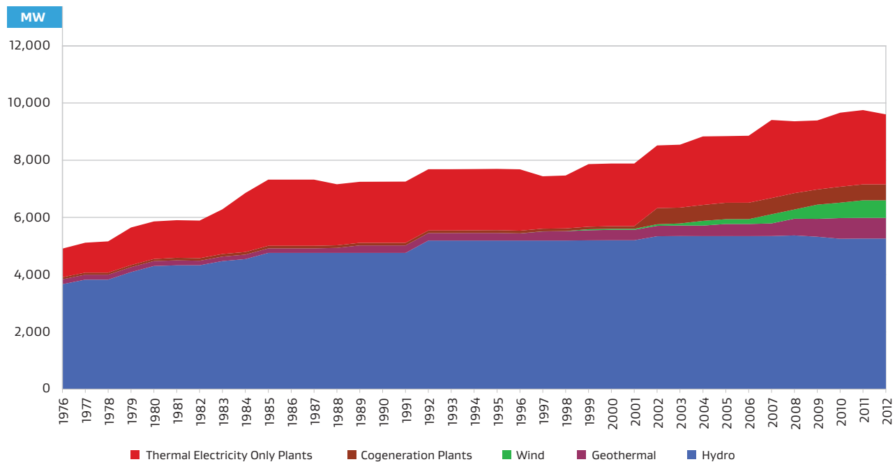
Figure F.2c: Operational Electricity Generation Capacity by Plant Type (MW)
