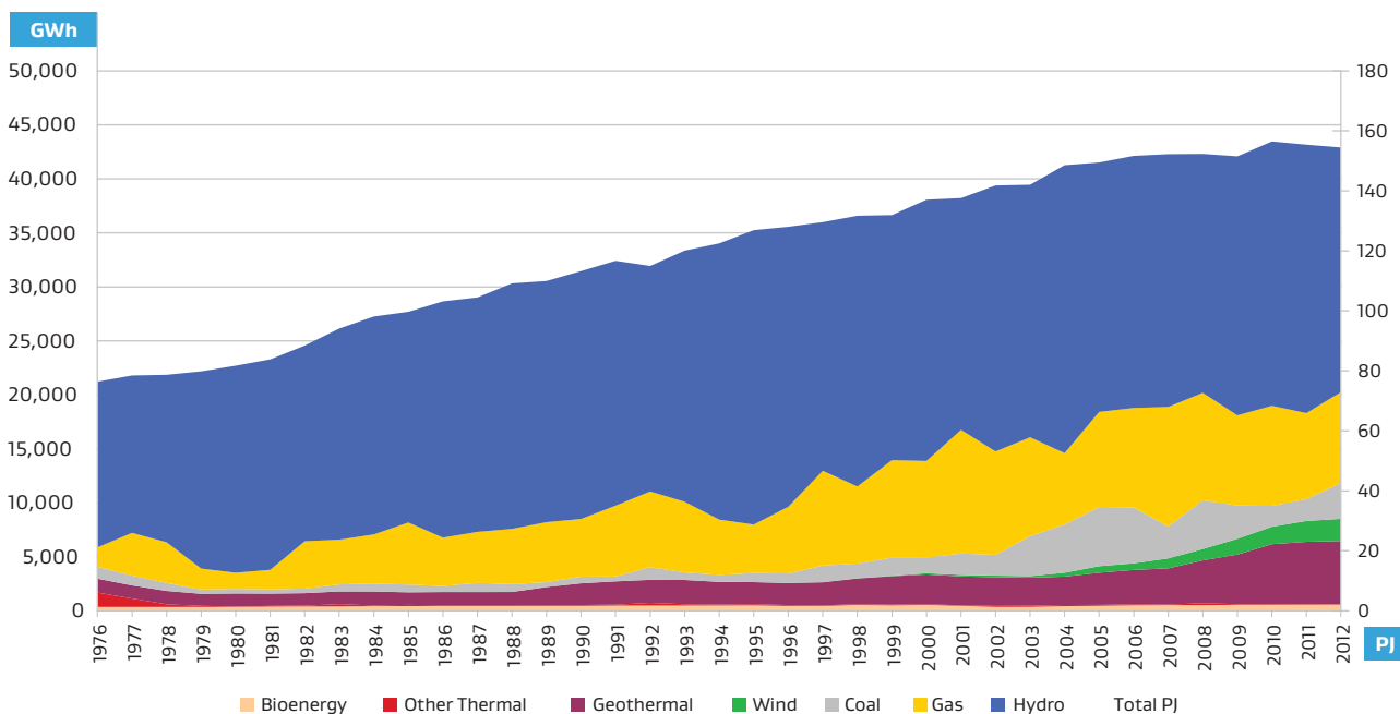
Figure F.2b: Annual Electricity Generation by Fuel Type
