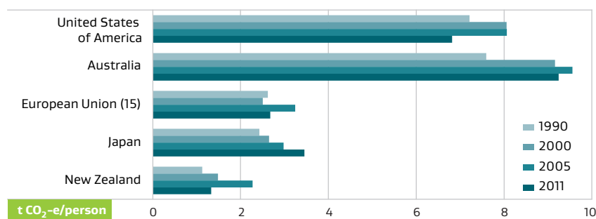
Figure A.5b: Electricity Generation Greenhouse Gas Emissions per Capita of Selected Annex 1 Countries 10
