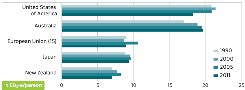
Figure A.5a: Energy Sector Greenhouse Gas Emissions per Capita of Selected Annex 1 Countries
