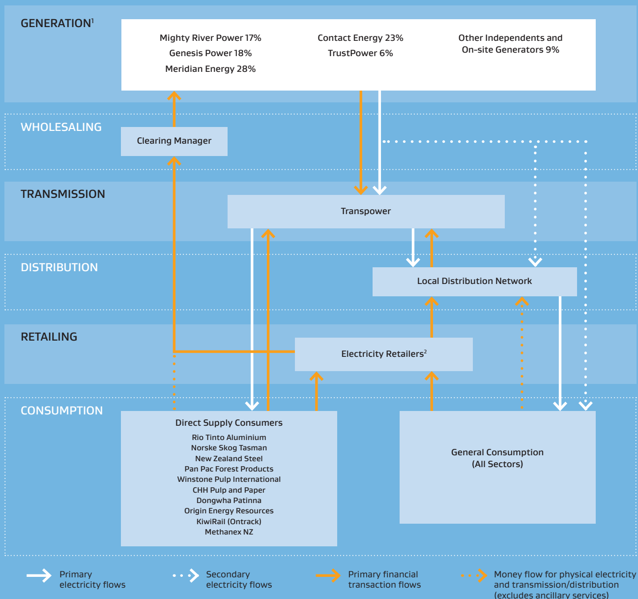
Figure F.1a: Electricity Industry Summary for 2012
