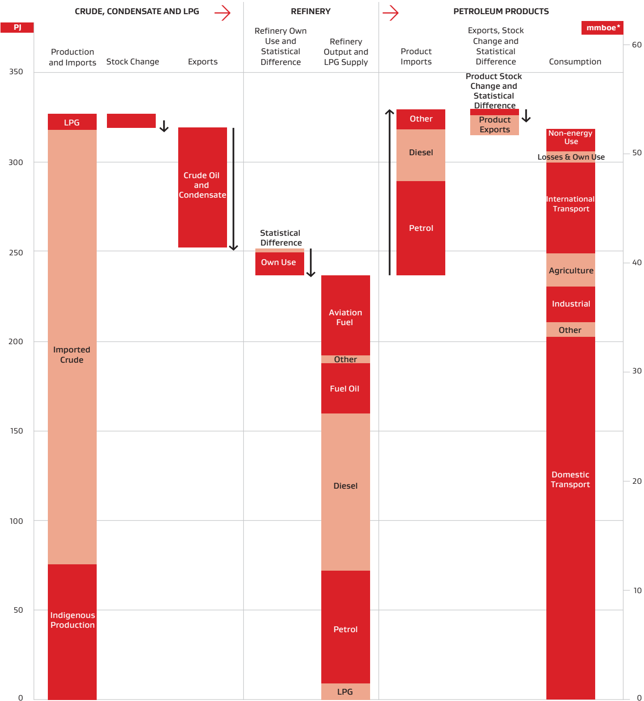
Figure D.4: Oil Energy Flow Summary for 2013
