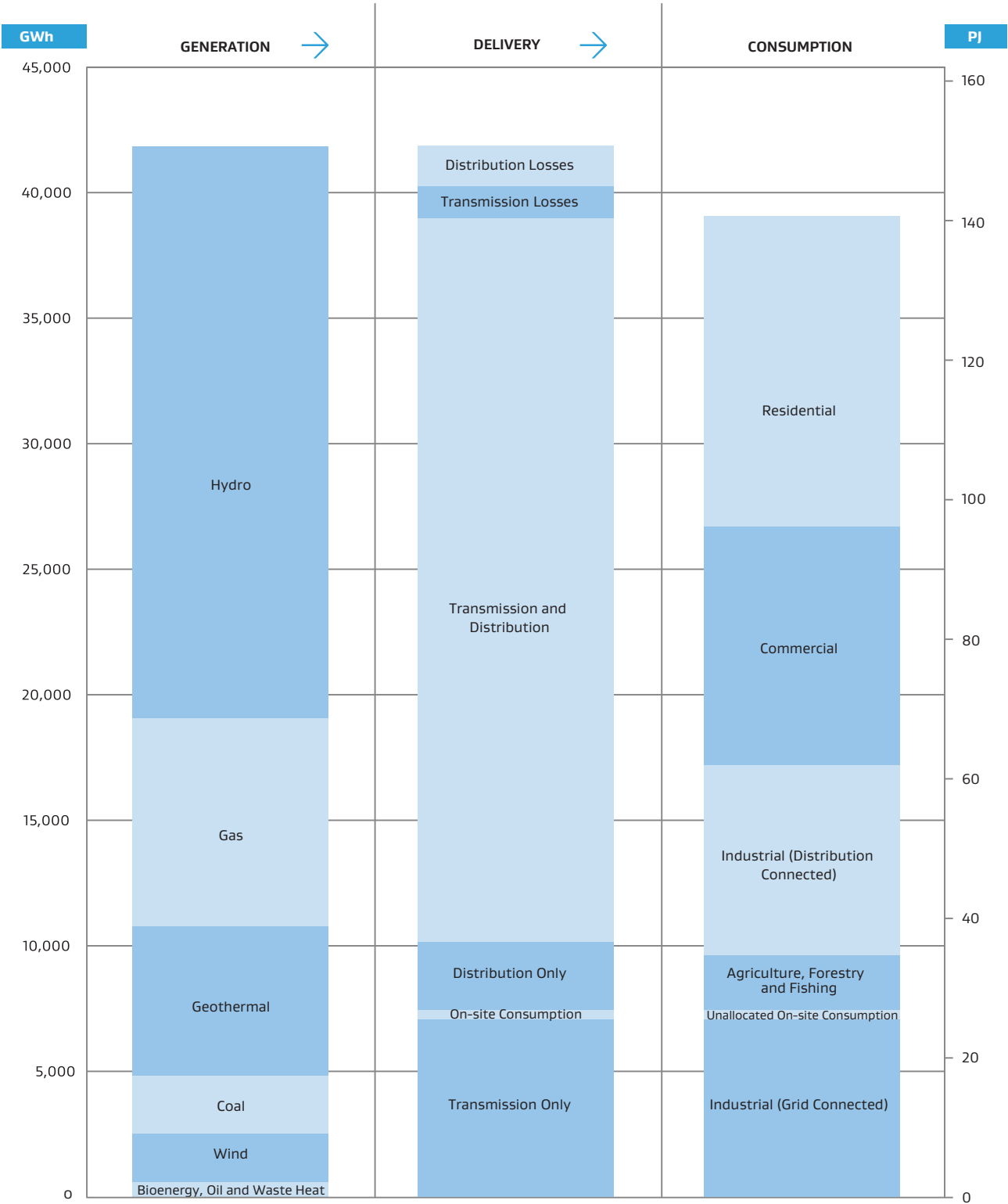
Figure F.2: Electricity Flow Diagram for the 2013 Year
