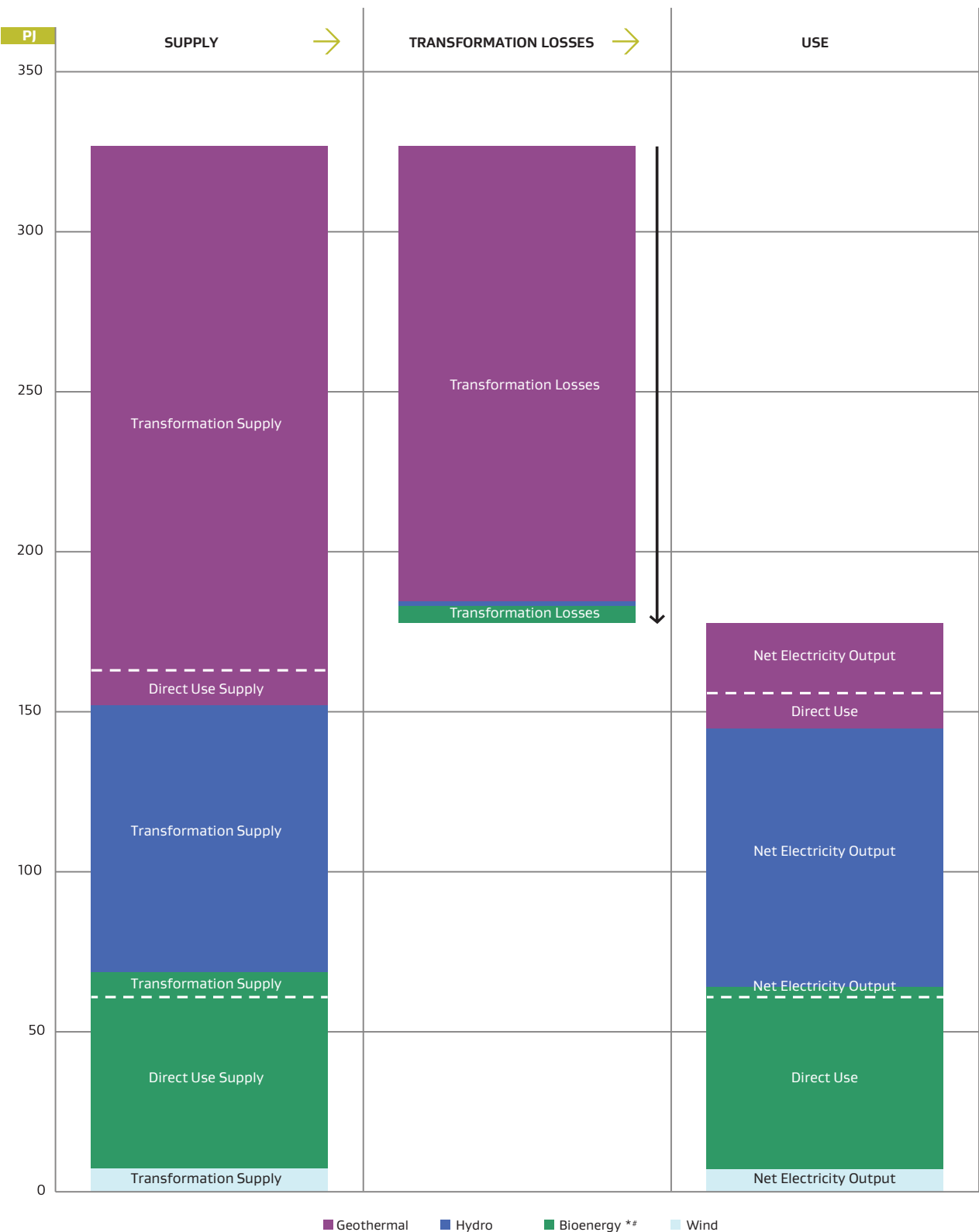
Figure E.1: Renewable Energy Flow Summary for 2013
